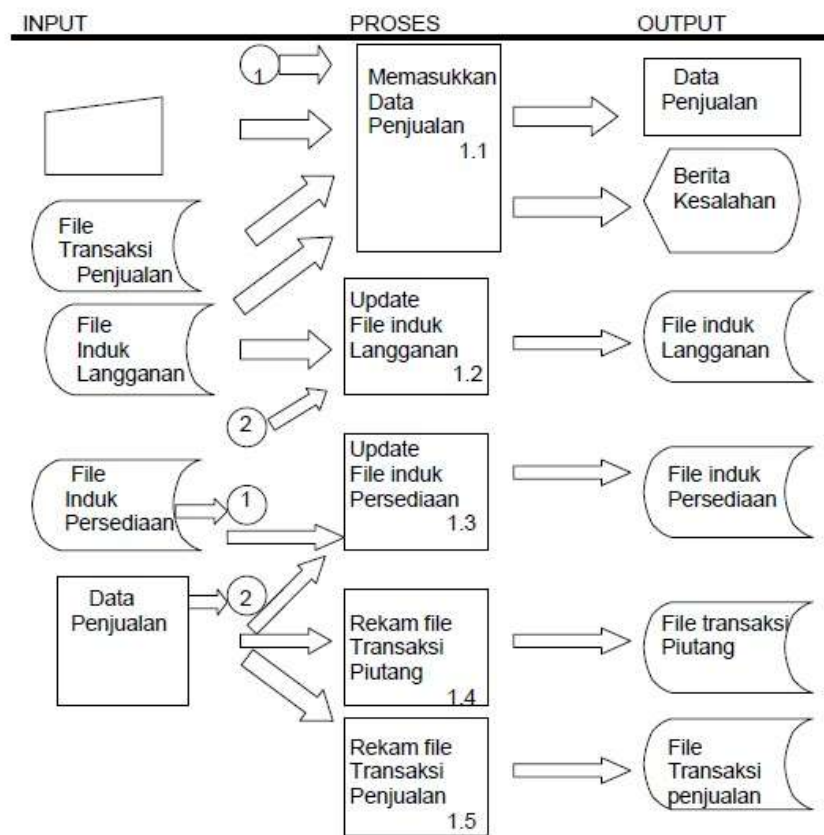
Gambar II.8 Overview Diagram (Sumber: Jogiyanto, 2005)
