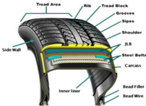
Figure 2 Virtual Tire Design (Source: Design from PT Hankook Tire)
